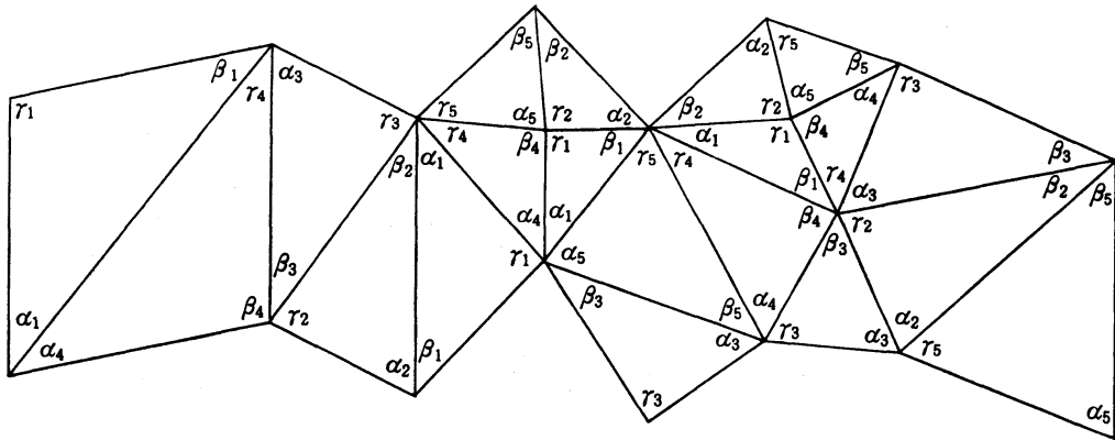
Developing map around the cusp
