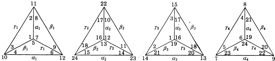
A nice triangulation of 6_1 - knot complement
