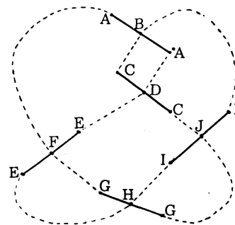
\partial D^- ( D^- is under this paper)
