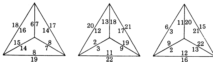
A nice triangulation of N .
