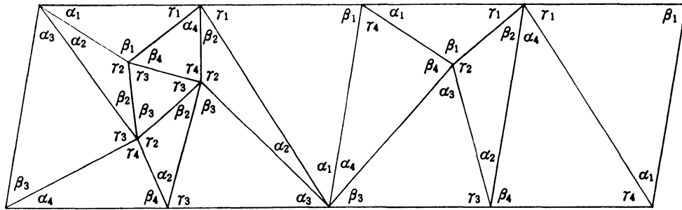
Developing map around the cusp
