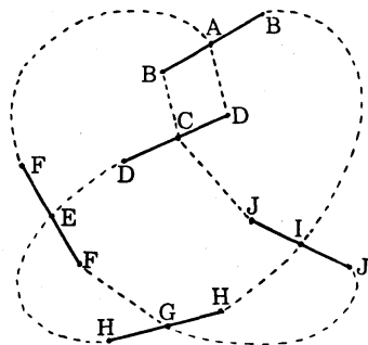
\partial D^+ ( D^+ is over this paper)
