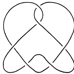
6_1 - knot (Stevedores knot)
