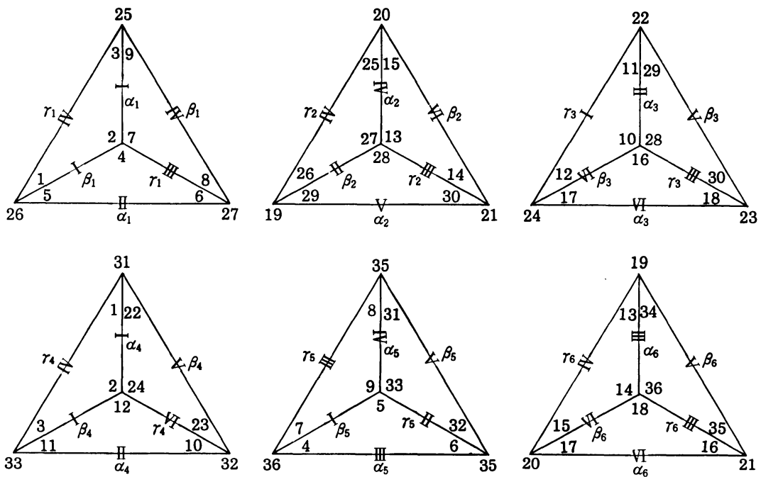
A nice triangulation of 6_3 - knot complement
