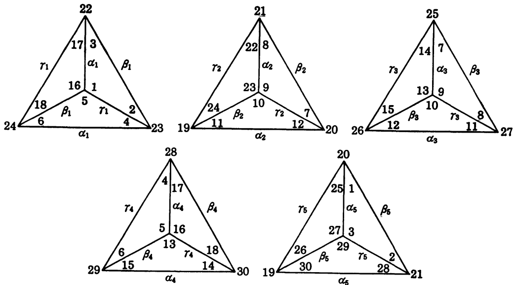
A nice triangulation of 6_2 - knot complement
