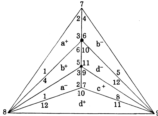
Polyhedron A
