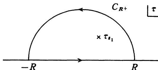
Figure 2. A path of integration
