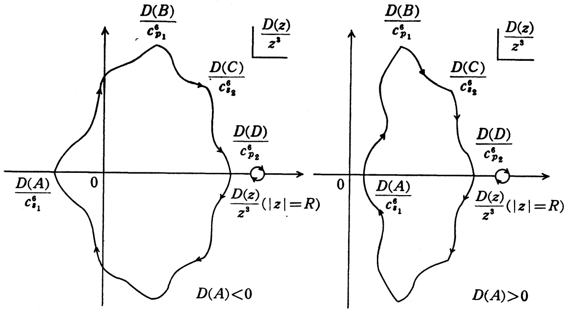
Figure 6. Path of the image point in the D(z)/z^3 -plane
