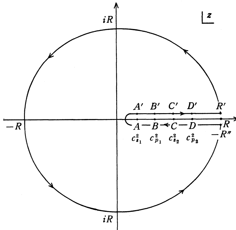
Figure 4. Path \gamma in the z plane
