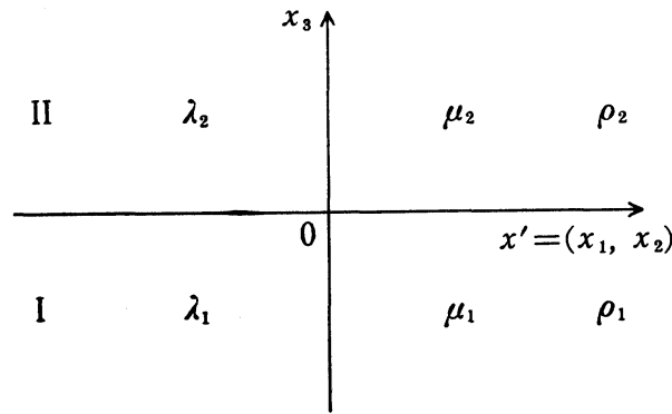
Figure 1. Stratified media I and II.
