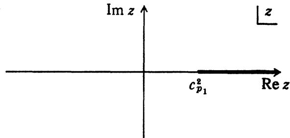
Figure 3. Branch cut between branch points c_{p_1}^2 and \infty in the z -plane
