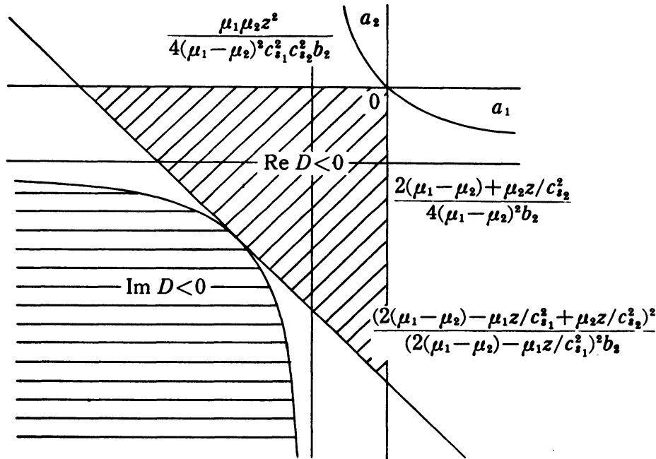
Figure 5. Behavior of \operatorname{Re} D(z) and \operatorname{Im} D(z) for variations of the parameters a_1 and a_2
