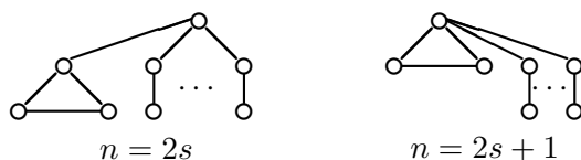
Figure 3. The graph D(n) .
