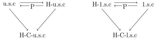
Figure 2.1: The relations between several types of upper/lower semicontinuity.
