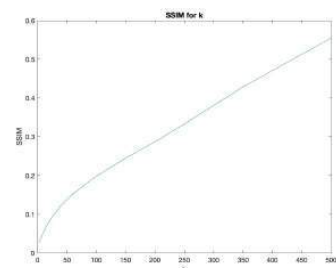
(c) SSIM
