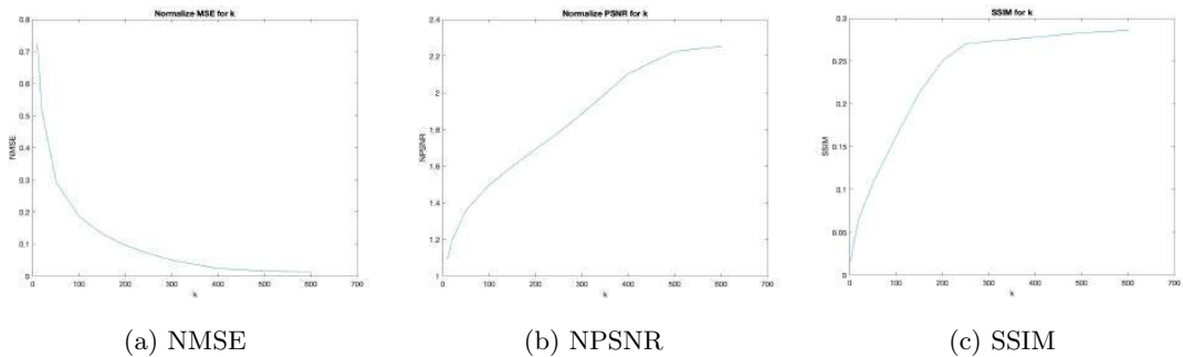
Figure 5.56: The diagram of curve for the image of “Fishing Boat” in the three measurements.
