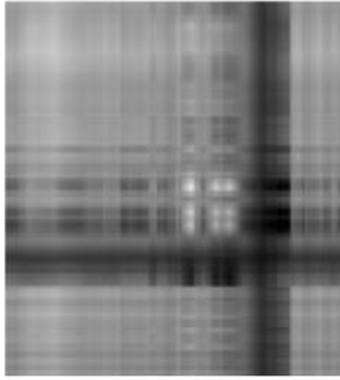
Figure 5.30: k = 2
