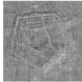
Figure 5.18: k = 21
