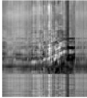
Figure 5.31: k = 11
