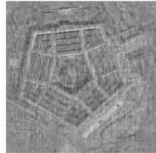
Figure 5.21: k = 50
