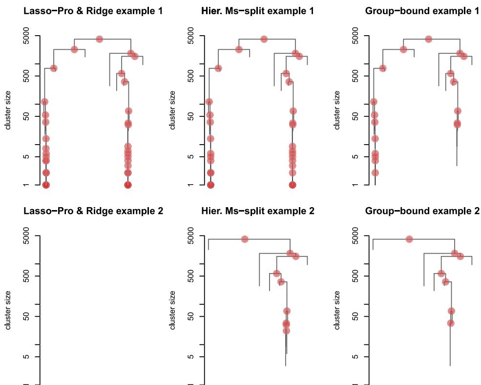
FIG. 8. A visualization of the hierarchical testing scheme as described in the beginning of Section 4, for the examples described in Section 4.4. One moves top-down through the output of a hierarchical clustering scheme, starting at the root node. For each cluster encountered, the null hypothesis that all the coefficients of that particular cluster are 0 is tested. A rejection is visualized by a red semi-transparent circle at a vertical position that corresponds to the size of the cluster. The chosen significance level was \alpha = 0.05 . The children of significant clusters in the hierarchy are connected by a black line. The process is repeated by testing the null hypotheses for all those children clusters until no more hypotheses could be rejected. The ordering of the hierarchy in the horizontal direction has no meaning and was chosen for a clean separation of children hierarchies. The hierarchical clustering and orderings are the same for all 6 plots since the design matrix was the same. Two different examples were looked at (corresponding to top and bottom row, resp.) and four different methods were applied to these examples. The desparsified Lasso and the Ridge method gave identical results and were grouped in the two plots on the left, while results from the hierarchical Multi sample-splitting method are presented in the middle column and the results for the Group-bound method are shown in the right column. In example 1, the responses were simulated with 2 clusters of highly correlated variables of size 3 having coefficients different from zero. In example 2, the responses were simulated with 2 clusters of highly correlated variables of sizes 11 and 21 having coefficients different from zero. More details about the examples can be found in Section 4.4.
