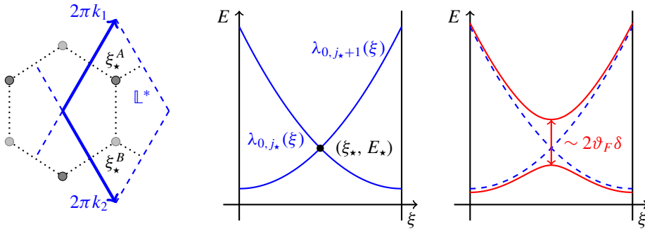
Figure 3. The picture on the left represents the Dirac points \xi_*^A and \xi_*^B inside a dual fundamental cell \mathbb{L}^* . The two pictures on the right represent the bifurcation of a Dirac point (\xi_*, E_*) to an open gap on a one-dimensional section of the Brillouin zone.
