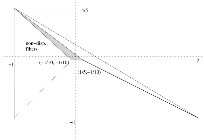
Figure 4. Orbifold \mathbb{P}(1, 3, 5)
