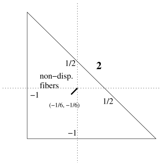
Figure 2. Orbifold \mathbb{P}(1, 2, 2)
