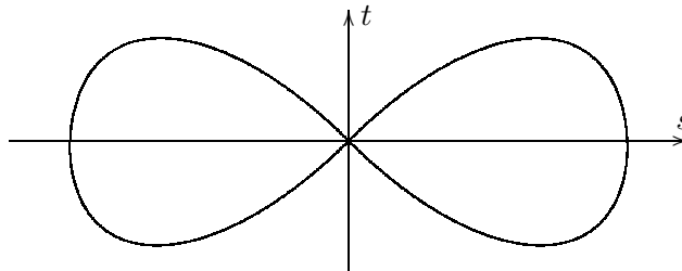
Figure 13.1. The curve C in \mathbb{C}
