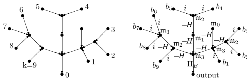
Figure 3.1. (a) A planar rooted tree (b) operators assigned to it
