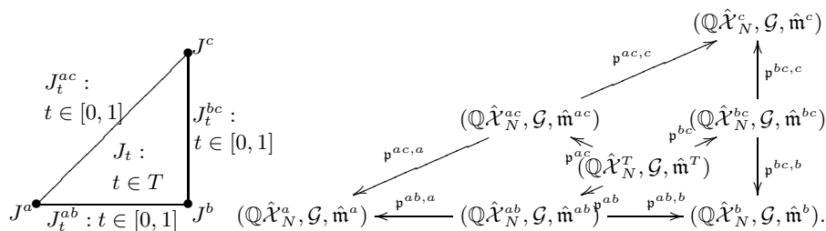
Figure 10.2. (a) J_t : t \in T (b) A_{N,0} algebras and morphisms
