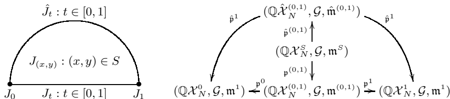
Figure 10.1. (a) J_s : s \in S (b) A_{N,0} algebras and morphisms
