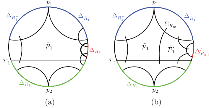
Fig. 9.3. (a) If D has more than 3 black regions, then, for a black region R_b distinct from R_1 and R_1^\pm , the open disk \text{int } \Delta_{R_b} is disjoint from |\text{BF}(p_1)| \cup |\text{BF}(p_2)| . (b) If D has precisely 3 black regions, then, for the black region R_{b,1} that is not adjacent to the white bigon R_w , the open disk \text{int } \Delta'_{R_{b,1}} , where \Delta'_{R_{b,1}} = \Delta_{R_{b,1}}(\tilde{\mathcal{P}}'_1) , is disjoint from |\text{BF}(p_1)| \cup |\text{BF}(p_2)| .
