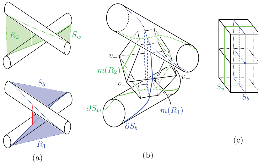
Fig. 6.2. At each crossing, (a) S_b and S_w intersect transversely along the crossing arc, (b) each of S_b and S_w intersects the partially truncated octahedron in a vertical middle plate containing the crossing arc, and (c) each of the middle plate determines a pair of midsquares in the pair of cubes, and the two pairs of midsquares intersect orthogonally along the vertical axes of the cubes.
