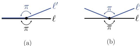
Fig. 6.4. Branching of geodesics. Though branching of geodesic can occur in CAT(0) spaces, it never occurs in Euclidean spaces.
