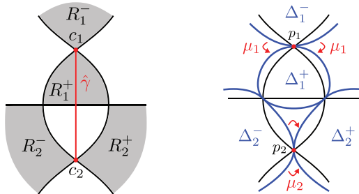
Fig. 9.4. The butterflies \text{BF}(p_1) and \text{BF}(p_2) and the actions of the meridians \mu_1 and \mu_2 , in the case \omega(\hat{\gamma}) > 0 . Here, we employ the model picture of the limit circles described in Remark 8.4 and Figure 8.1.
