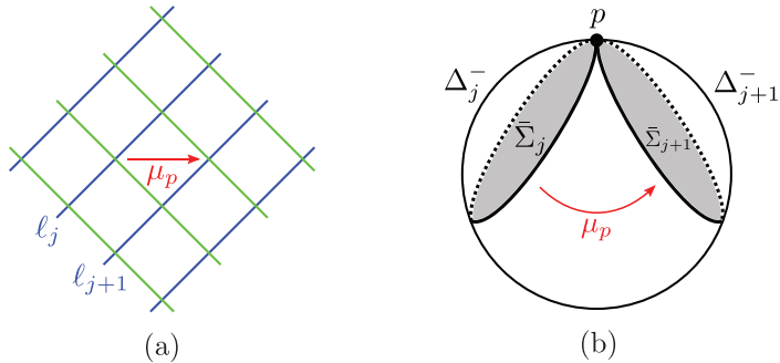
Fig. 4.1. (a) The action of \mu_p on (H_p, H_p \cap p_u^{-1}(S_b), H_p \cap p_u^{-1}(S_w)) . (b) A rough model of the action of \mu_p on (\mathbb{H}^3, \{\bar{\Sigma}_j\}_j) . This figure is not precise. In fact, \Delta_j^- \cap \Delta_{j+1}^+ = \partial \Delta_j^- \cap \partial \Delta_{j+1}^+ is generically strictly bigger than \{p\} (cf. Remark 4.8).
