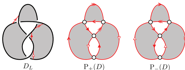
Fig. 7.1. The decomposition of the figure-eight knot complement into a pair of checkerboard ideal polyhedra: The shaded regions are black regions and the unshaded regions are white regions.
