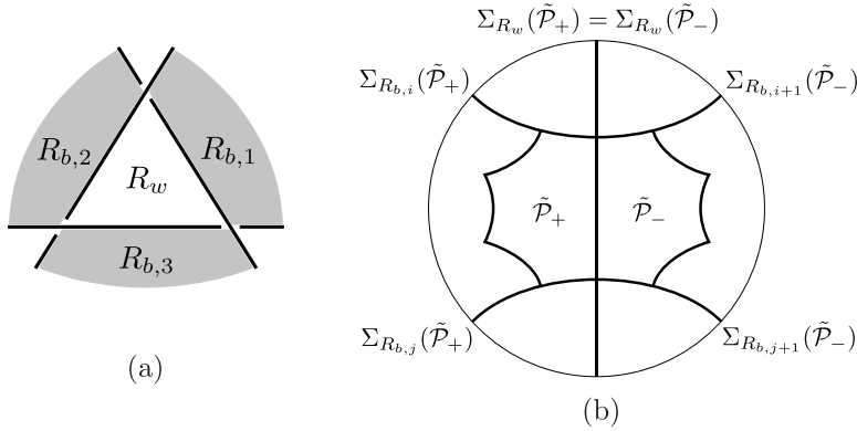
Fig. 7.3. The checkerboard polyhedra \tilde{\mathcal{P}}_+ and \tilde{\mathcal{P}}_- share a face that is contained in the checkerboard hyperplane \Sigma_{R_w}(\tilde{\mathcal{P}}_+) = \Sigma_{R_w}(\tilde{\mathcal{P}}_-) . Then \Sigma_{R_{b,i}}(\tilde{\mathcal{P}}_+) = \Sigma_{R_{b,i+1}}(\tilde{\mathcal{P}}_-) .
