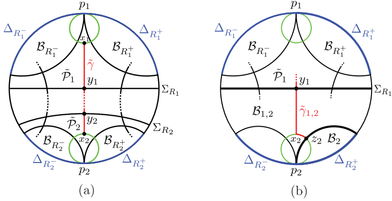
Fig. 9.2. (a) The checkerboard hyperplane \Sigma_{R_1}(\tilde{\mathcal{P}}_1) separates \mathcal{B}_{R_1^-} \cup \mathcal{B}_{R_1^+} and \mathcal{B}_{R_2^-} \cup \mathcal{B}_{R_2^+} . Note that \mathcal{B}_{R_1} = \mathcal{B}_{R_1}(\tilde{\mathcal{P}}_1) is the region in \tilde{\mathcal{X}} = \mathbb{H}^3 “below” \Sigma_{R_1} . (b) The arc \tilde{\gamma}_{1,2} , that is the union of the arc \delta \subset H_{p_2} and the subarc of \tilde{\gamma} bounded by y_1 and x_2 , intersects \Sigma_{R_1} and \Sigma_{R_2^\epsilon} only at the endpoints. Here \epsilon = + .
