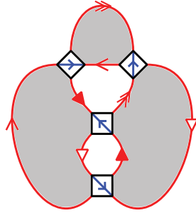
Fig. 8.2. The truncation \tilde{\mathcal{P}}_0 of the checkerboard ideal polyhedron \tilde{\mathcal{P}} = \tilde{\mathcal{P}}_+ . The blue diagonal arcs in the squares project to meridians.
