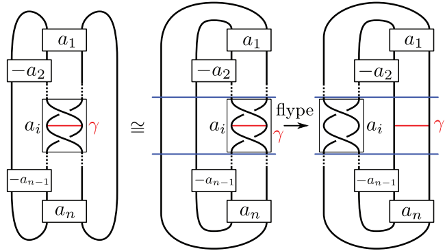
Fig. 9.8. If i is even, then first modify D by an ambient isotopy in S^2 into the middle diagram and then apply the flype.
