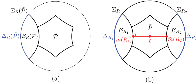
Fig. 7.2. (a) \mathcal{B}_R(\tilde{\mathcal{P}}) is the checkerboard half-space in \tilde{\mathcal{X}} bounded by the hyperplane \Sigma_R(\tilde{\mathcal{P}}) which is disjoint from \text{int } \tilde{\mathcal{P}} . (This 2-dimensional figure does not reflect the fact that \tilde{\mathcal{P}} is an ideal polyhedron.) (b) If R_1 and R_2 are not adjacent, then \angle_{\tilde{v}}(\tilde{m}(R_1), \tilde{m}(R_2)) = \pi , and hence [\tilde{m}(R_1), \tilde{v}] \cup [\tilde{v}, \tilde{m}(R_2)] is a common perpendicular to \Sigma_{R_1} and \Sigma_{R_2} . This implies \mathcal{B}_{R_1}(\tilde{\mathcal{P}}) \cap \mathcal{B}_{R_2}(\tilde{\mathcal{P}}) = \emptyset .
