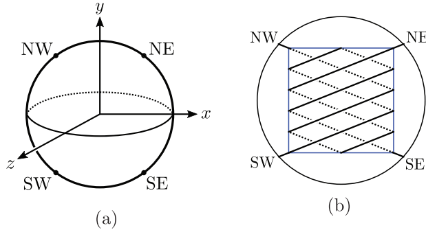
Fig. 10.1. (a) The 3-ball \mathbf{B}^3 with the set P^0 of the four marked points. (b) The rational tangle (\mathbf{B}^3, t(r)) with r = 2/5 . Note that the vertical axis is the y -axis, not the z -axis.
