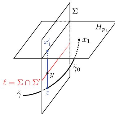
Fig. 9.1. If a checkerboard hyperplane \Sigma' \neq \Sigma intersects [x'_1, z] , then it separates H_{p_1} and z , and hence intersects \tilde{\gamma}_0 .
