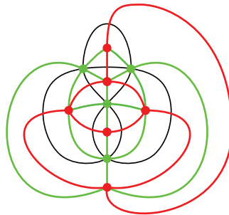
Fig. 6.3. The geometric link \text{Lk}(v_\epsilon, \mathcal{M}) : The union of the thick red graph and the thick green graph forms the 1-skeleton of \text{Lk}(v_\epsilon, \mathcal{M}) .
