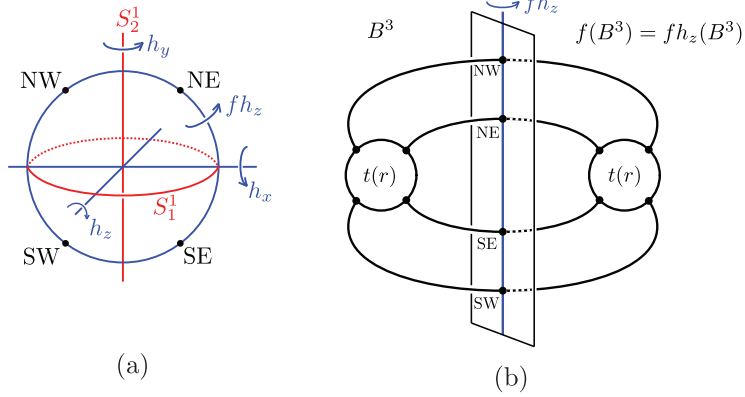
Fig. 10.2. In (a), the axis of the \pi -rotation fh_z is the great circle \partial B^3 \cap \{z = 0\} , and it passes through the four marked points. In (b), \partial B^3 is the central vertical plane and the axis of fh_z is the vertical line. The free involution f is the composition of the \pi -rotations fh_z and h_z , where \text{Fix}(fh_z) \cup \text{Fix}(h_z) forms a Hopf link.
