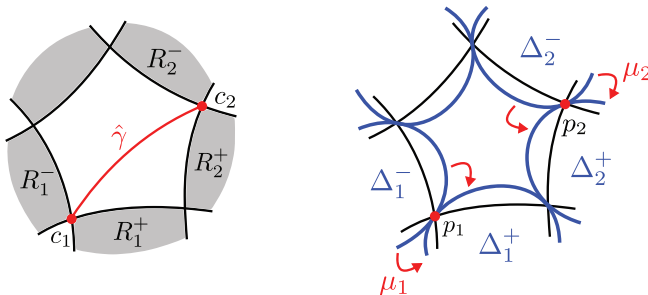
Fig. 9.5. The butterflies \text{BF}(p_1) and \text{BF}(p_2) and the actions of the meridians \mu_1 and \mu_2 , in the case \omega(\hat{\gamma}) = 0 and \gamma is not a crossing arc. Here, we employ the model picture of the limit circles described in Remark 8.4 and Figure 8.1.
