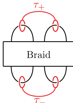
Fig. 1.1. The upper and lower meridian pairs of a 2-bridge link group. The proper arcs \tau_+ and \tau_- in the exterior M(L) of a 2-bridge link L \subset S^3 are the upper and lower tunnels, respectively. Each of the meridian pairs represented by \tau_+ and \tau_- generates the link group G(L) = \pi_1(S^3 \setminus L) .
