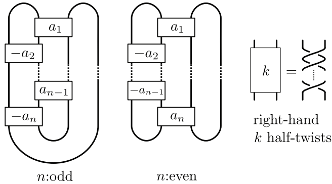
Fig. 9.6. The standard prime alternating diagram D of a hyperbolic 2-bridge link L .
