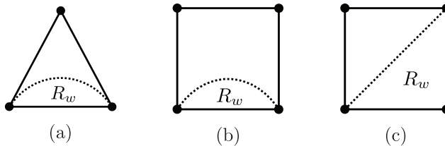
Fig. 8.3. The plane graph \mathcal{G} dual to the black regions. The complementary region of \mathcal{G} labeled R_w determines the desired white region R_w .
