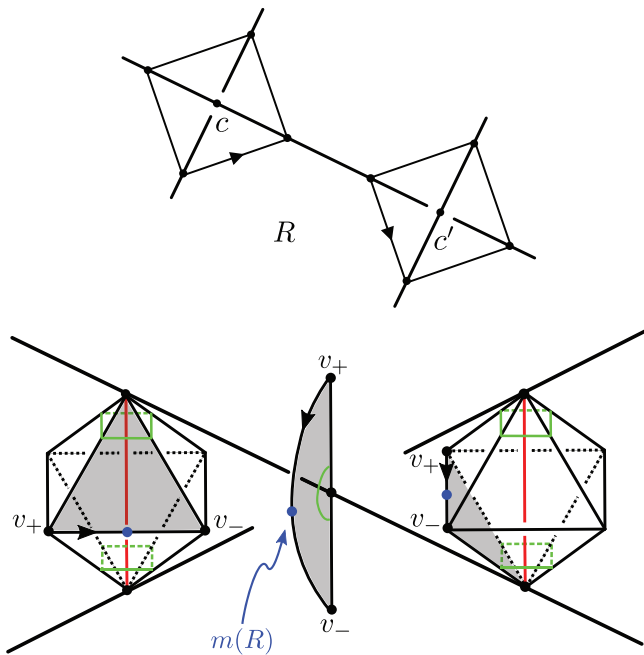
Fig. 6.1. Local picture of the cubed complex \mathcal{M} . The partially truncated octahedra in M are expanded so that they cover the whole M . The shaded faces of the octahedra at the crossings c and c' are identified with the central bow-shaped face. In particular, the pair of the horizontal arrowed edges of the octahedra are identified with the arrowed edge of the bow-shaped face joining monotonically the top vertex v_+ and the bottom vertex v_- , passing through the center m(R) of the region R .
