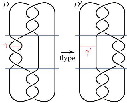
Fig. 9.7. The flype maps the crossing arc \gamma in the diagram D to an arc which is not a crossing arc in the new diagram D' .
