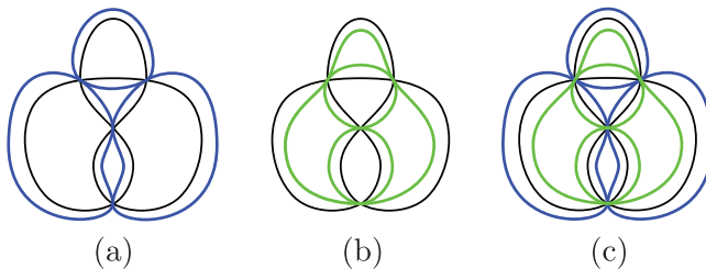
Fig. 8.1. Put a circle C_R around each region R of the diagram D , so that C_R bounds a disk containing R and passes through the vertices on \partial R . The figures (a) and (b) illustrates the circles \{C_R\} where R runs over the black or white regions, respectively. By overlaying these two figures, we obtain the figure (c). According to [3], the figure (c) “illustrates” the intersection pattern of the limit circles \{\partial_\infty(\Sigma_R(\tilde{\mathcal{P}}))\}_R , where R runs over the regions of D .
