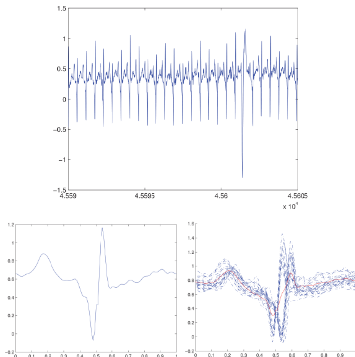
FIG 1. Top: Original time series “chfdb chf13 45590” of the ECG dataset; Bottom left: One individual cycle; Bottom right: whole cycles (in dashed blue) and the average cycle (in red).
