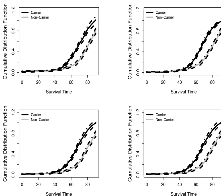
FIG 4. Distribution of the age-at-death for huntingtin gene mutation carriers and non-carriers in COHORT: estimated CDFs (solid) and the 95% confidence band (upper band dot-dashed, lower band dashed). Upper Left: Ignore within-family correlation (MW; Assuming independence as in Ma and Wang (2014) [11]); Upper Right: Treat within-family correlation (CWLS); Lower left: BLRE.
