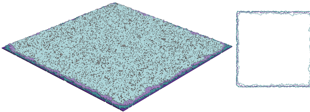
Figure 1: An Ising interface in \Lambda_n for n = 500 conditioned to lie above a floor at height h = 0 .
