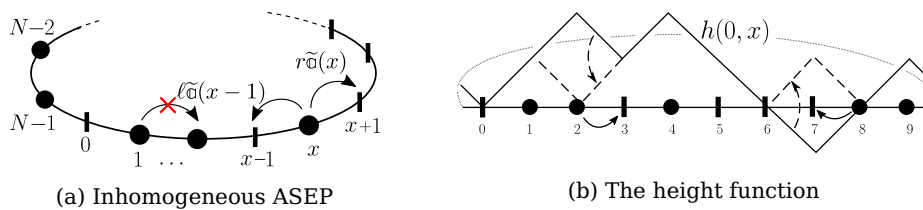
Figure 1: Inhomogeneous ASEP on \mathbb{T} and its height function. (a): The particle at x jumps to x - 1 at rate \tilde{\omega}(x - 1)\ell or to x + 1 at rate \tilde{\omega}(x)r ; meanwhile the particle at 1 may not jump to the occupied site 2. (b): The particle dynamics are coupled with a height function as shown.
