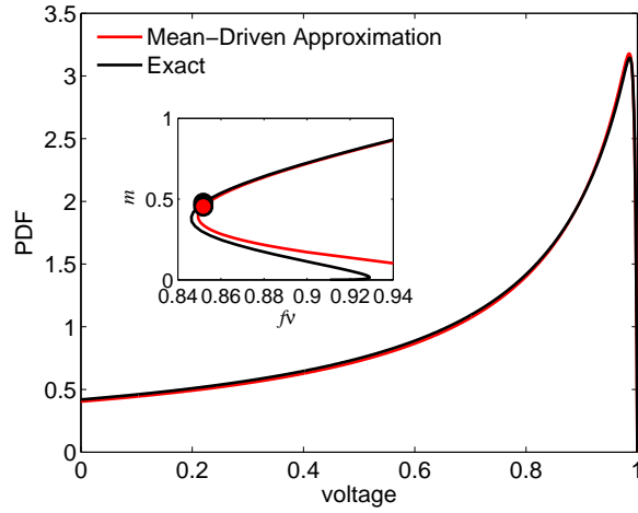
FIG. 4.7. Comparison between the exact voltage PDF in (4.24) (black) and its mean-driven approximation in (4.33) (dark grey, red online) near the lower turning point of the gain curve. The two gain curves are shown in the inset. The parameter values are f = 0.001 , S = 0.6 and N = 1000 .
