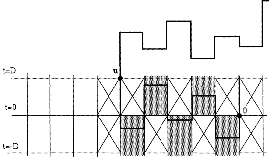
Fig. 3. A schematic representation of the local event \mathcal{E}_1 used in the proof of Theorem 7.6. Crossed areas do not contain any bonds and gray areas contain at least one bond
