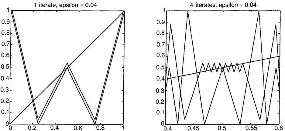
Fig. 1. The fourth iterate of a map with a fixed turning point compared to the fourth iterate of a perturbation
