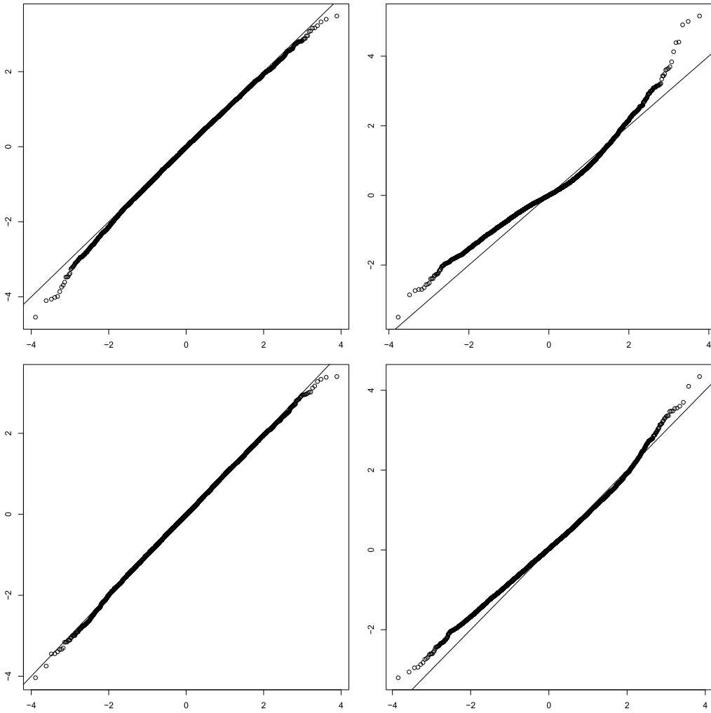
Figure 4. QQ-plots comparing \widehat{Z}_{G,n} (left) and \widehat{Z}_{H,n} (right) to the \mathcal{N}(0, 1) distribution in the case of the non-ergodic model (4.3) for n = 10^3 (above) and n = 10^4 (below).
