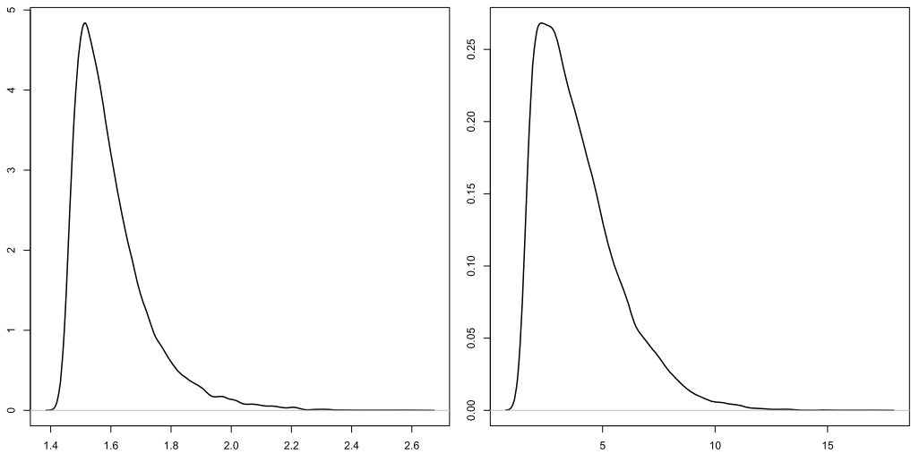
Figure 2. Approximation to the densities of W_G(\theta_0) (left) and W_H(\theta_0) (right) based on \tilde{W}_G and \tilde{W}_H in the case of the ergodic model (4.1).
