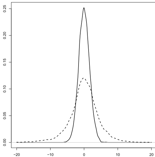
Figure 3. Estimated densities of \sqrt{n}(\hat{\theta}_{G,n} - \theta_0) (solid curve) and \sqrt{n}(\hat{\theta}_{H,n} - \theta_0) (dashed curve) for n = 10^4 in the case of the ergodic model (4.1).
