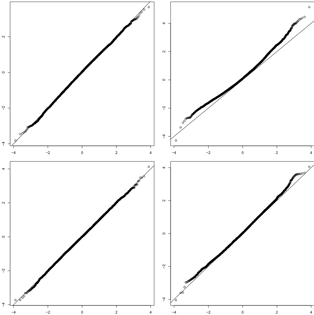
Figure 1. QQ-plots comparing \widehat{Z}_{G,n} (left) and \widehat{Z}_{H,n} (right) to the \mathcal{N}(0, 1) distribution in the case of the ergodic model (4.1) for n = 10^3 (above) and n = 10^4 (below).
