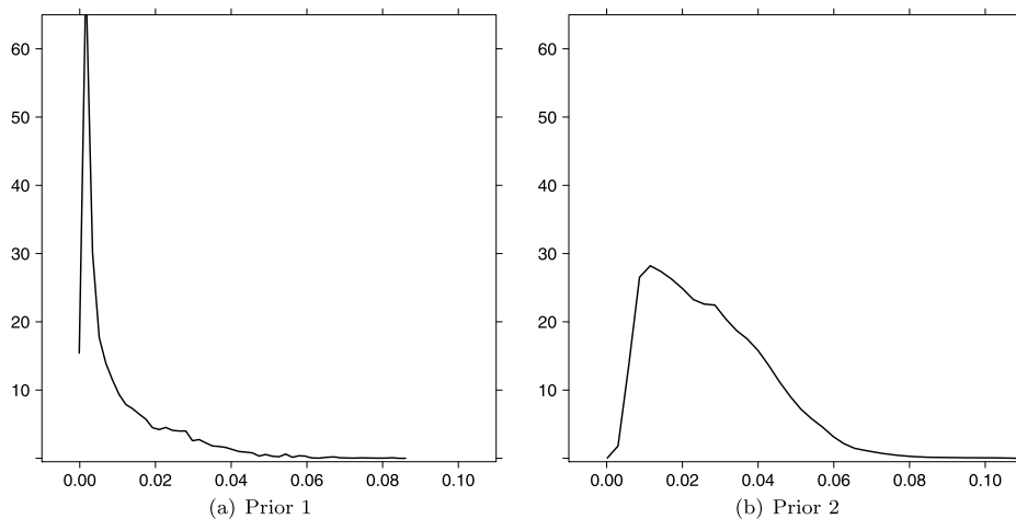
Figure 8: For each of the priors of Figure 1, the posterior credence density of the length of the uncertainty interval for PC*, conditional on the lower bound being greater than 0.
