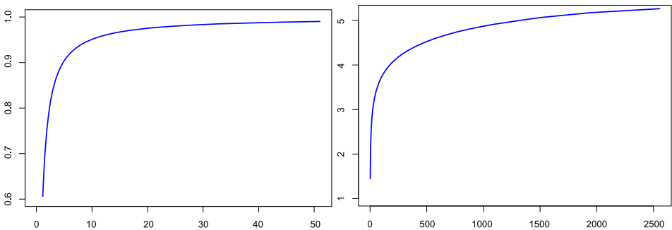
FIG. 2. The plots of mappings \gamma \mapsto z_\gamma and \gamma \mapsto l_\gamma(z_\gamma) . One can observe that both functions are increasing, the first one converges to 1 very rapidly, while the second one seems to diverge very slowly.
