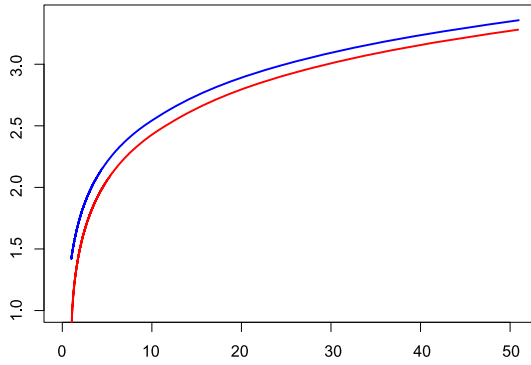
FIG. 4. The curves of functions L \mapsto l_L(z_L) (blue curve) and L \mapsto l_{\gamma_L}(z_{\gamma_L}) (red curve).
