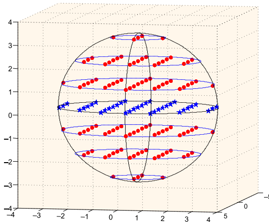
FIG. 1. Lattice points in a ball of radius R = \gamma d^* = 3.2 in the three dimensional space ( d^* = 3 ). Red points are those of \mathcal{C}_1(d^*, \gamma) \setminus \mathcal{C}_2(d^*, \gamma) while blue stars are those of \mathcal{C}_2(d^*, \gamma) . In this example, N(d^*, \gamma) = N(3, 1.07) = 110 .
