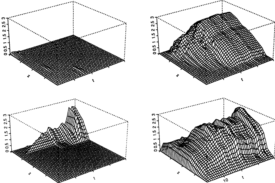
FIG. 2. The test process \hat{J}(X) for the BMRC data (first row) and the corresponding untransformed process X (second row). Positive parts are on the left; negative parts are on the right.
