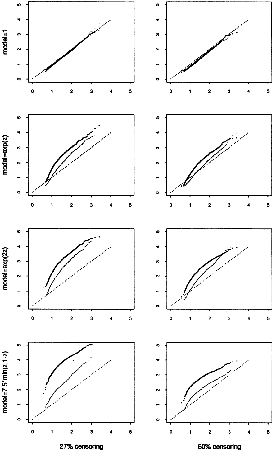
FIG. 1. Q-Q plots of the observed distribution of S against the distribution of S^* at sample sizes 500 (thick lines) and 1000 (thin lines).
