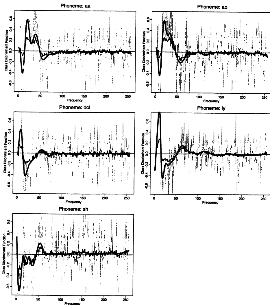
FIG. 6. Class discriminant functions for the five phonemes: these are analogs of the functions \Sigma_W^{-1} m^j for linear discriminant analysis, except the within covariance here is penalized. The thick solid curve represents PDA using the improper spline penalty and 30 df . The raw LDA coefficients are in the background. The wiggly curve is the ridge version of PDA, using 70 df .
