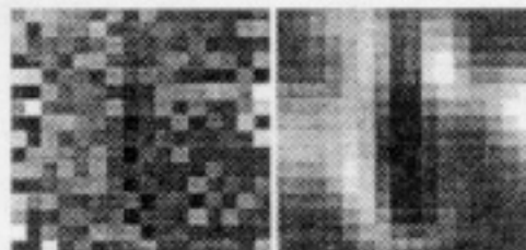
LDA: Coefficient 1
