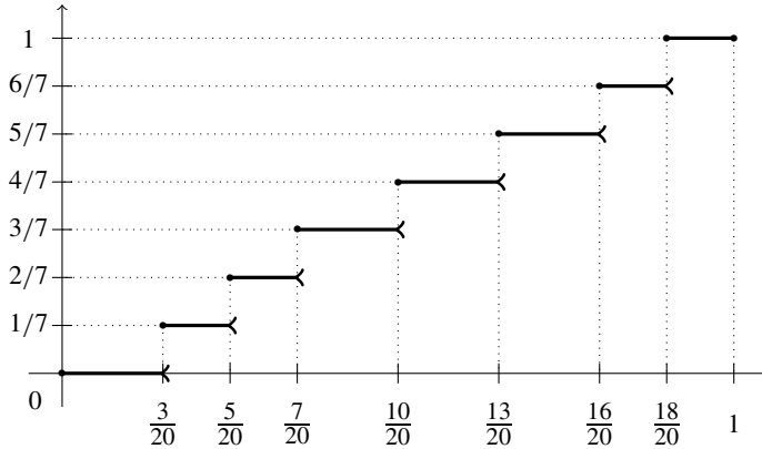
FIG. 10. The leaf distribution function F_t for the tree t shown in Figure 7. Note that F_t is piecewise constant and all gaps are of height \frac{1}{|t|} (here, \frac{1}{7} ), but pieces may have different widths (here, \frac{2}{20} or \frac{3}{20} ). Informally, Proposition 3.5 states that these widths are asymptotically close to each other.
