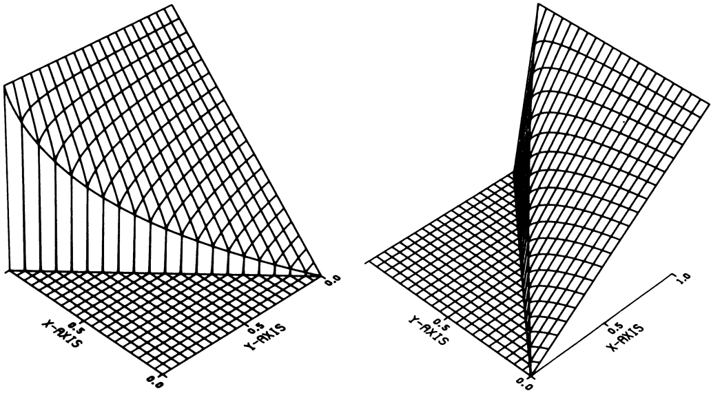
FIG. 1. The limit function L from two viewpoints.
