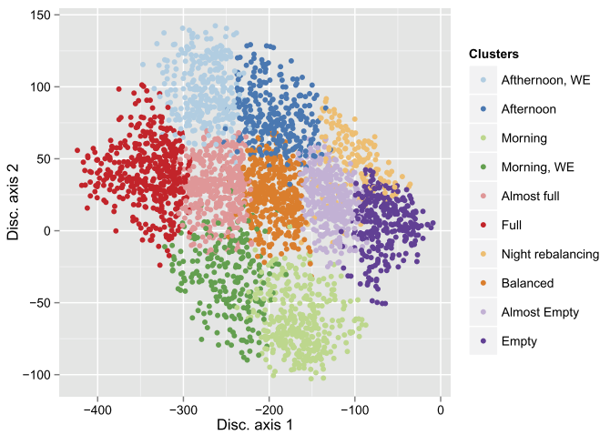
FIG. 14. Bike stations projected into the two first axes of the discriminative functional subspace. Colors indicate the cluster memberships.
