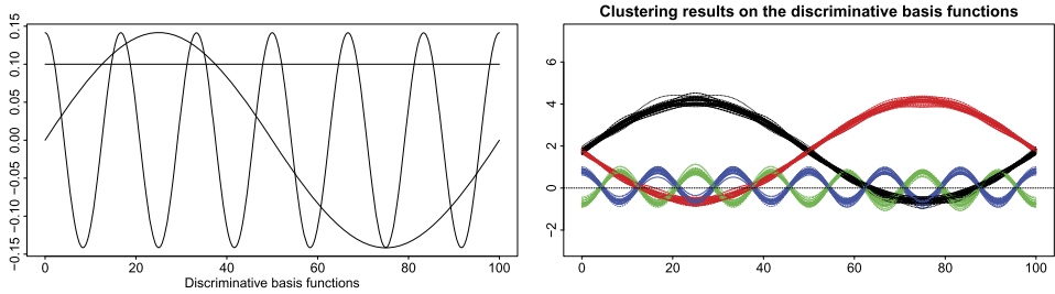
FIG. 8. Discriminative functions among the Fourier basis functions: selected basis functions (left) and data projected on the selected basis functions (right).
