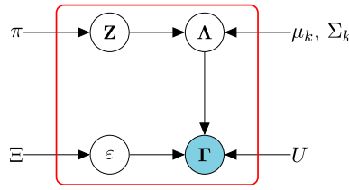
FIG. 3. Graphical representation for the model DFM_{[\Sigma_k \beta]} .
