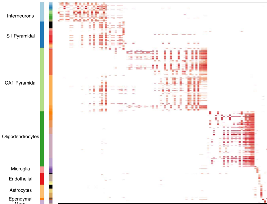
(b) Factor matrix found by ISA.
