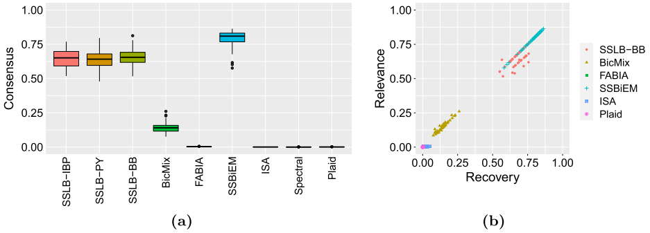
FIG. 7. Simulation 2: (a) Boxplots of the consensus scores. (b) Relevance versus recovery scores.
