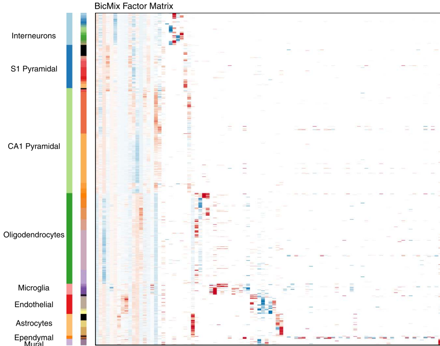
(a) Factor matrix found by BicMix.
