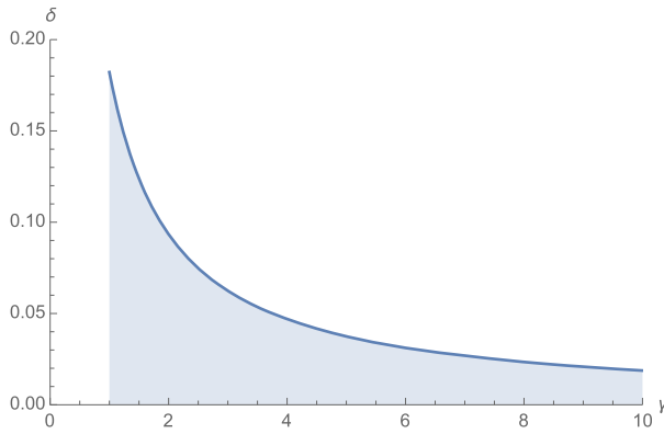
FIG. 1. The good set G_2 embedded in the upper right quadrant of \mathbb{R}^2 .
