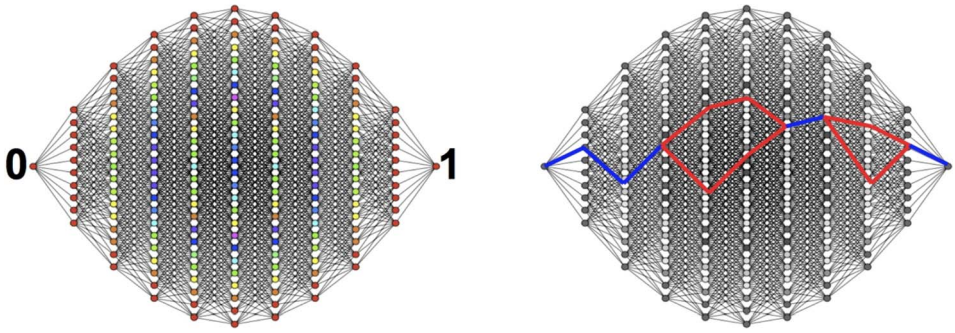
FIG. 1. The 10-dimensional hypercube (left), and two oriented connecting paths (right). Blue edges are common to both paths, whereas paths do not overlap on red edges.
