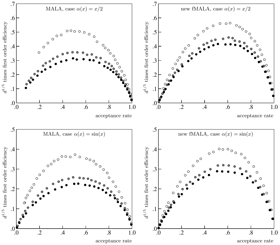
FIG. 4. First-order efficiency of the new fMALA and the standard MALA as a function of the overall acceptance rates for the dimensions d = 100 (white points), d = 500 (gray points), d = 1000 (dark points), respectively, for the nonproduct density (45) with \alpha(x) = x/2 (top pictures) and \alpha(x) = \sin(x) (bottom pictures).
