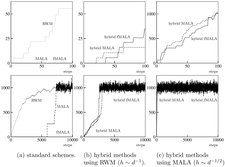
FIG. 2. Trace plots of \|X\|^2 for the Gaussian target density in dimension d = 1000 when starting at the origin. Comparison of fMALA with h \sim d^{-1/5} (solid lines), MALA with h \sim d^{-1/3} (dashed lines), RWM with h \sim d^{-1} (dotted lines).
