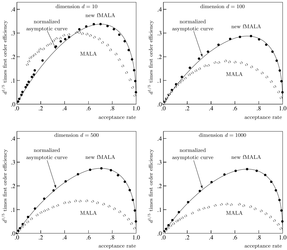
FIG. 1. First-order efficiency of the new fMALA and the standard MALA for the double well potential g(x) = -\frac{1}{4}x^4 + \frac{1}{2}x^2 , as a function of the overall acceptance rates in dimensions d = 10, 100, 500, 1000 . The solid line is the reference asymptotic curve of efficiency for the new fMALA, normalised to have the same maximum value as the finite dimensional fMALA.
