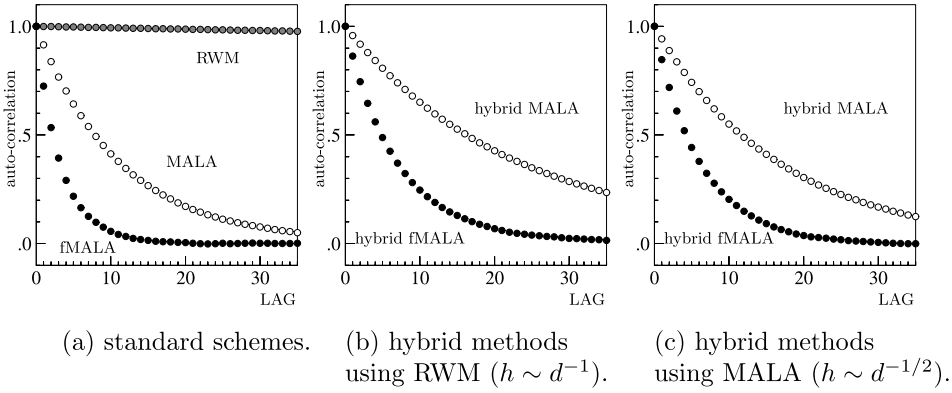
FIG. 3. Auto-correlation versus LAG for the Gaussian target density in dimension d = 1000 . Comparison of fMALA with h \sim d^{-1/5} (black), MALA with h \sim d^{-1/3} (white), RWM with h \sim d^{-1} (gray).
