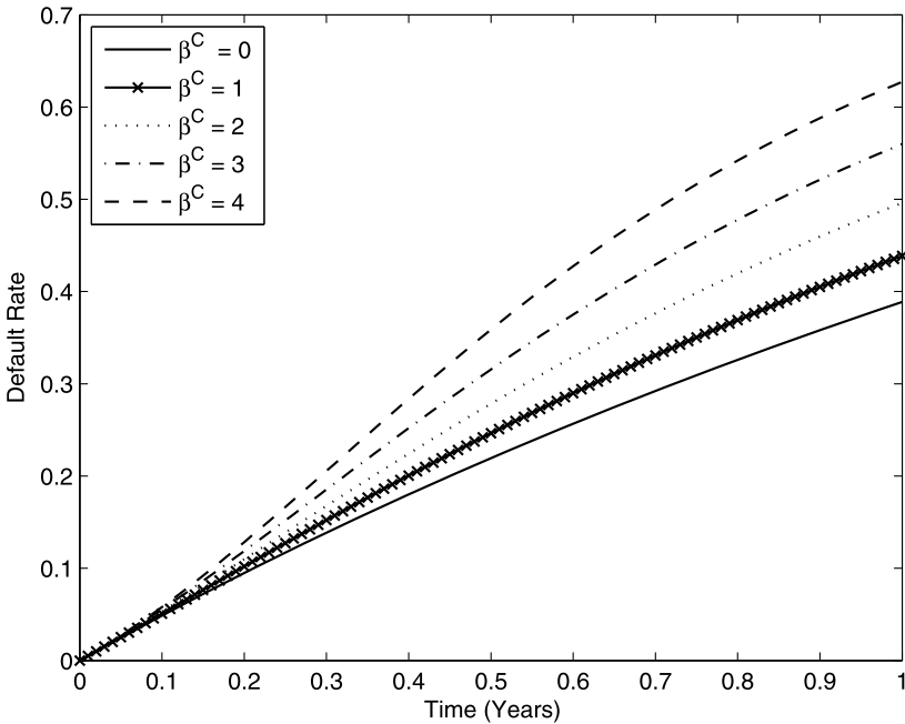
FIG. 1. Comparison of limiting default rate F(t) for different values of the contagion sensitivity \beta^C . The parameter case is \sigma = 0.9 , \alpha = 4 , \bar{\lambda} = 0.5 and \lambda_0 = 0.5 .
