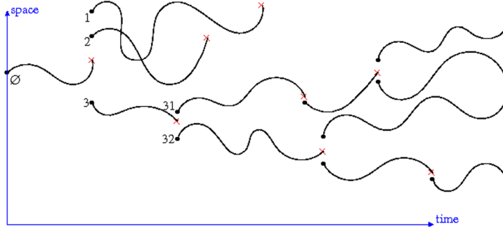
FIG. 2. Continuous time Markov process indexed by the Galton–Watson tree of Figure 1.
