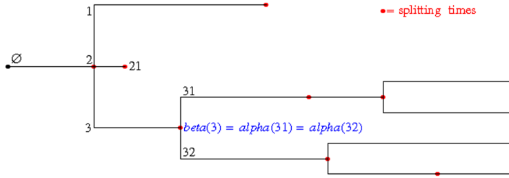
FIG. 1. Continuous time Galton–Watson tree.
