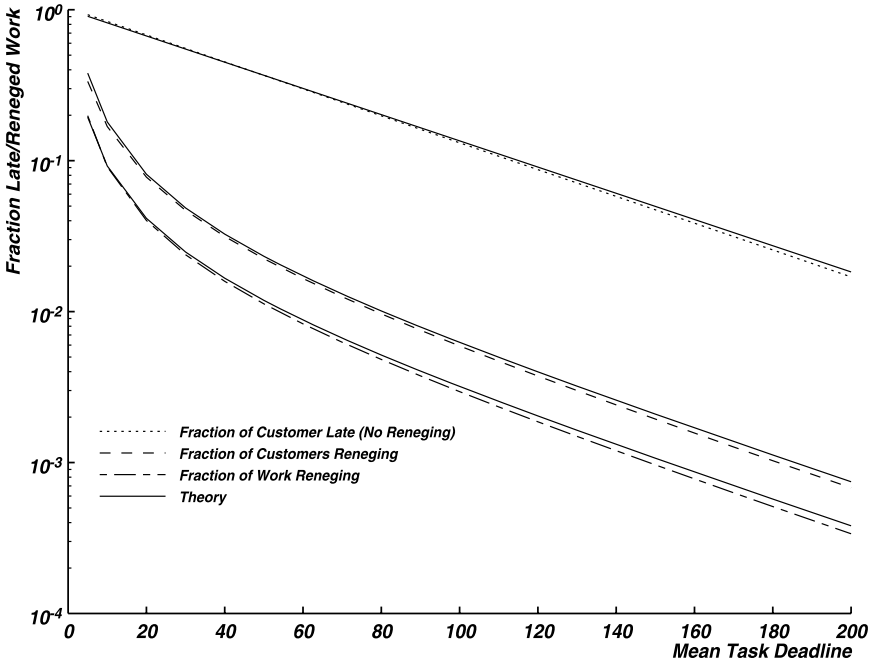
FIG. 2. M/D/1 queue.
