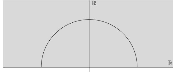
Fig. 2. The upper half-plane in Euclidean space \mathbb{R}^{n+1} (shaded) and the upper hemisphere \mathbb{S}_+^n .
