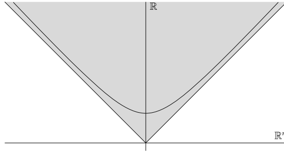
Fig. 1. Minkowski space \mathbb{R}^{n,1} . The shaded area is the causal future and the hyperboloid is \mathbb{H}^n .
