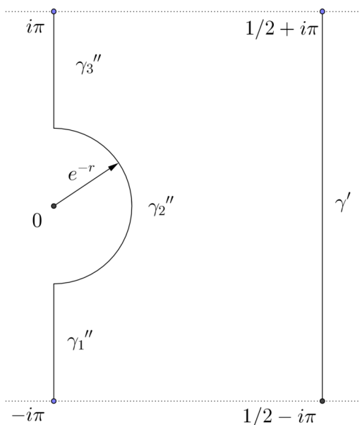
Fig. 1. The contours \gamma' and \gamma'' .
