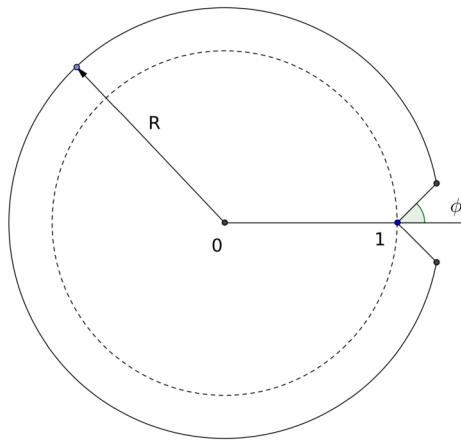
Fig. 2. Illustration of \Delta_0 .
