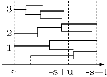
Fig. 2. At a fixed time -s , three families are present, they will all die out at time -s + t . M_{-s}^{-s+u} equals the number of bold lines present at any time -s + u . Then the total lifetime of the population at -s is to add the length of the bold parts together.
