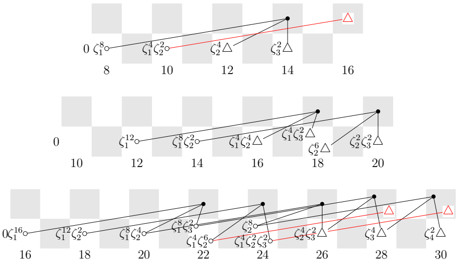
Figure 1: v_0^{-1} \text{Ext}_{E(2)*}(\Sigma^8 \underline{\text{bu}}_2) (top), v_0^{-1} \text{Ext}_{E(2)*}(\Sigma^{12} \underline{\text{bu}}_3) (middle) and v_0^{-1} \text{Ext}_{E(2)*}(\Sigma^{16} \underline{\text{bu}}_4) (bottom)
