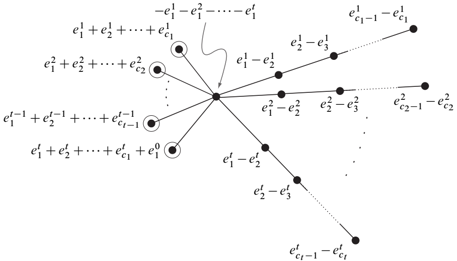
Figure 8: Up to a change of basis the embedding of the canonical negative plumbing graph for the family (p1) : the basis of \mathbb{Z}^m is \{e_1^0, e_j^k\} , where k \in \{1, \dots, t\} and j \in \{1, \dots, c_k\} .
