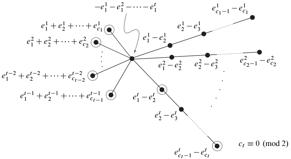
Figure 9: Up to a change of basis the embedding of the canonical negative plumbing graph for the family (\mathbf{p2}) , where c_t > 0 is the only even parameter: the basis of \mathbb{Z}^m being \{e_j^k\} where k \in \{1, \dots, t\} and j \in \{1, \dots, c_k\} .
