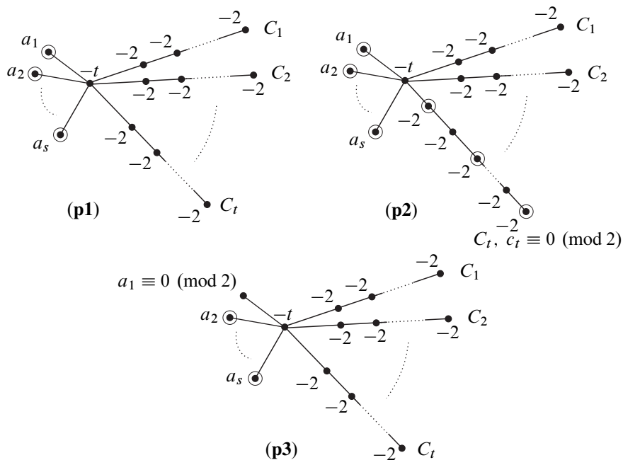
Figure 4: Wu-set on canonical negative plumbing graphs corresponding to the pretzel knots in families (p1), (p2) and (p3).
