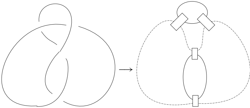
Figure 8: Example of a non-alternating B -adequate knot diagram
