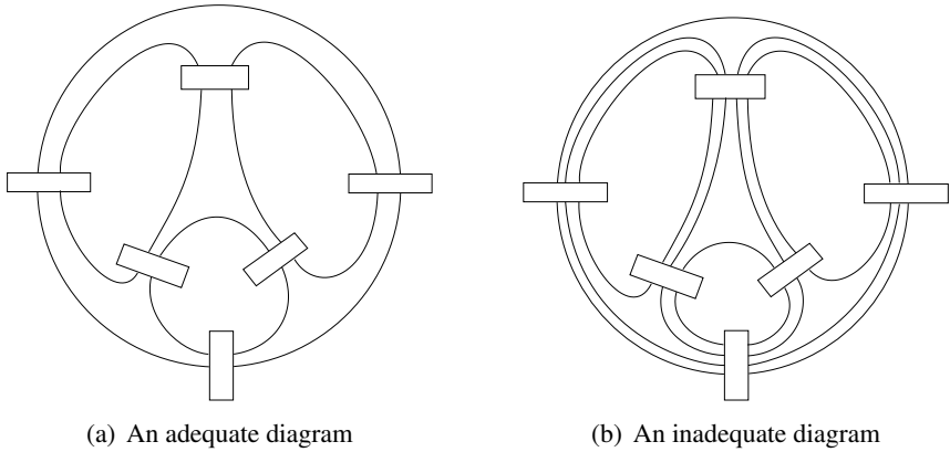
Figure 3: Example of adequate and inadequate diagrams
