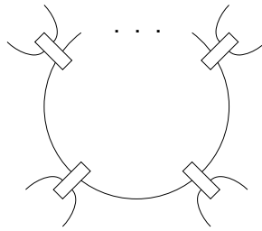
Figure 5: A circle from S_B seen in S_B^{(n+1)}
