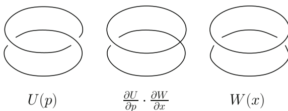
Figure 19: The three boundary configurations.
