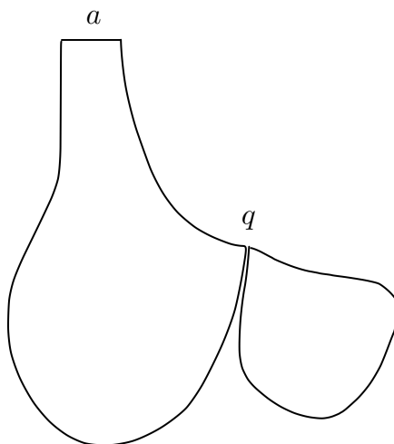
Figure 14: In the presence of double points, disks with one puncture at the double point can break off, leading to new codimension-one boundary phenomena that can destroy the chain map property.
