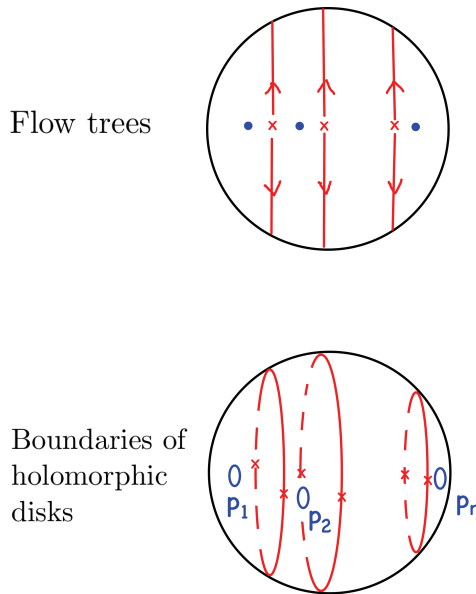
Figure 18: The flow trees that correspond to rigid disks, and the boundaries of the corresponding rigid disks lying in a fiber punctured sphere of N_{K/K_1} .
