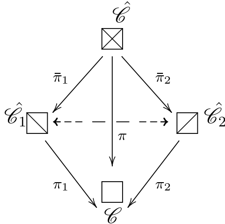
Figure 8: Flop transition \hat{\mathcal{C}}_1 \longleftrightarrow \hat{\mathcal{C}}_2 between the two small resolutions of the conifold.
