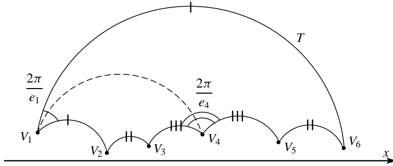
Fig. 1. A general Klein tile T for s = 4
