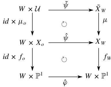
Fig. 14. Commutative diagram (vi)
