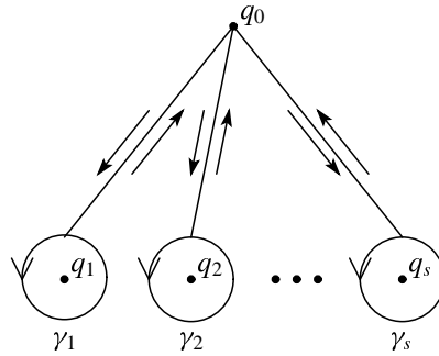
Fig. 3. The meridians
