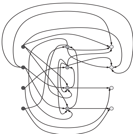
Figure 8. The network arising from a two-point star.
