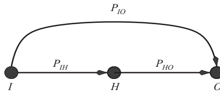
Figure 1. The simplest network.
