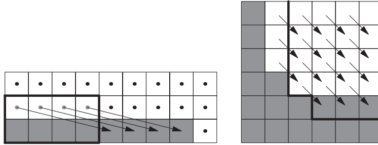
FIGURE 1. The arrow maps of Example 3.1.
