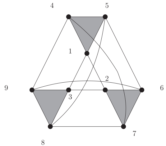
FIGURE 6. The T -graph of 2 points in \mathbb{P}^2 .
