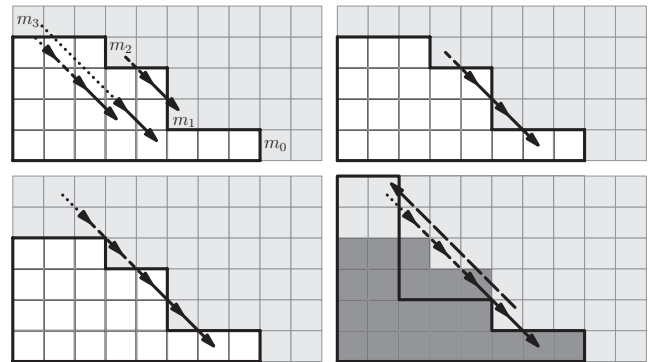
FIGURE 4. The upper left picture shows the path c_2^1 c_1^1 from m_2 and the paths c_3^1 c_1^1 and c_3^1 c_2^1 c_1^1 from m_3 ; the upper right picture shows the walk c_2^1 c_1^1 c_1^1 from m_2 ; the lower left the stroll c_3^1 c_2^1 c_2^1 c_1^1 c_1^1 from xy^5 ; the lower right the hike \tilde{c}_1^1 c_3^1 c_2^1 c_2^1 c_1^1 c_1^1 from x^5y to x^6 .
