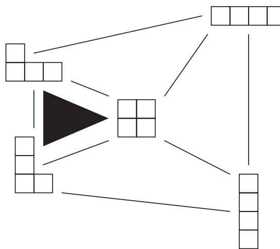
FIGURE 5. The T -graph of four points in \mathbb{A}^2 .
