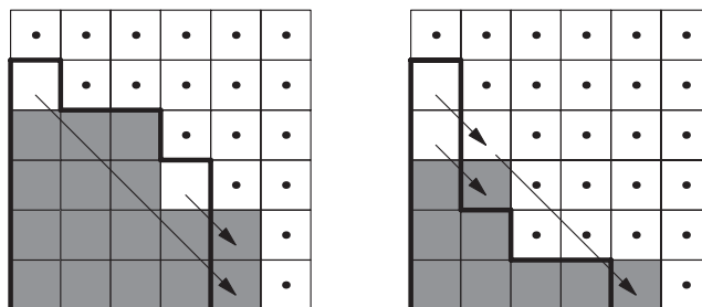
FIGURE 2. The arrow maps and systems of arrows of Example 3.8.
