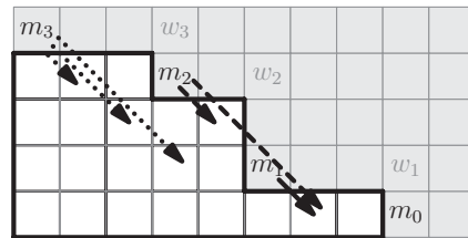
FIGURE 3. The positive significant arrows for the monomial ideal \langle x^8, x^5y, x^3y^3, y^4 \rangle of Example 4.3. Here c_1^1 is solid, c_2^1, c_2^3 are dashed, and c_3^1, c_3^2, c_3^3 are dotted.
