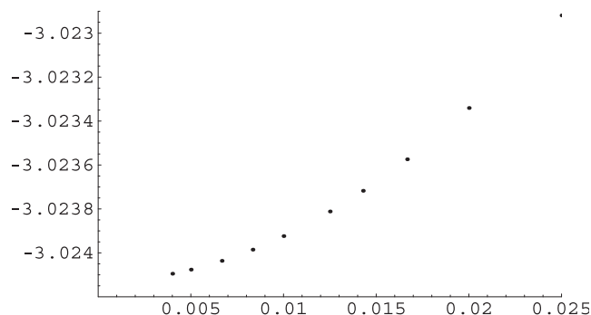
FIGURE 8. Dots indicate (1/N, 2\pi \operatorname{Im} \log(J_{N+1}(5_2)/J_N(5_2))) for N = 40, 50, 60, 70, 80, 100, 120, 150, 200, 250 . The origin corresponds to (0, -3.0242) .
