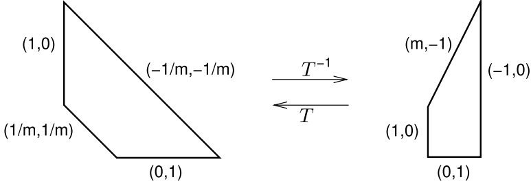
Figure 1. Hirzebruch surfaces.
