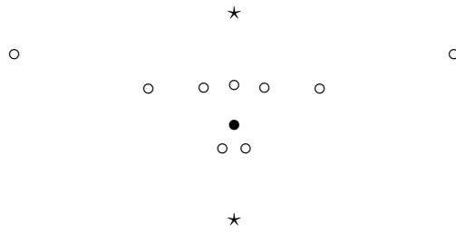
Figure 7: Configuration of type (1, 9, 2) with c_3 = 20/3 , X \simeq .17786964i .
