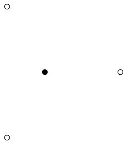
Figure 2: The Costa Hoffman Meeks configuration, m = 3 .
