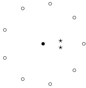
Figure 10: Configuration of type (1, 9, 2) with c_3 = 10^{-3} , X \simeq 1.961678 .
