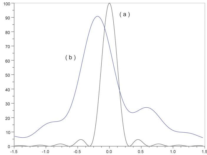
Figure 2: Comparison of the emitted radiation lineshape between (a) the case with only the solenoid and (b) the case where also an electric field is present.
