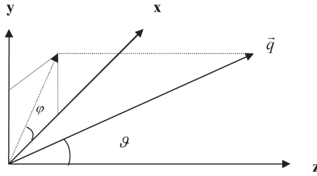
Figure 1: Reference frame definition for (8.2). The magnetic field is directed along the z -axis.
