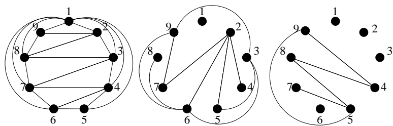
FIGURE 1. A minimum planar decomposition of K_9 .
