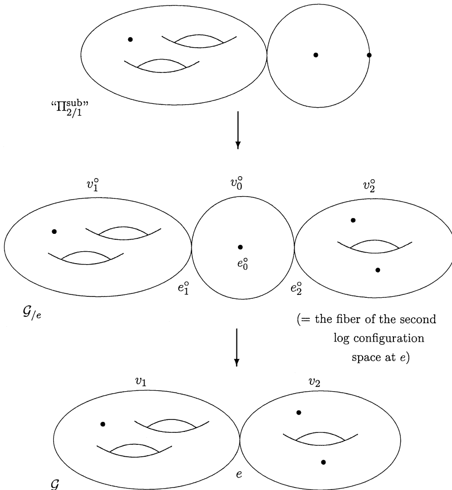
Fig. 1. \mathcal{G} , \mathcal{G}/e , and “ \Pi_{2/1}^{\text{sub}} ”
