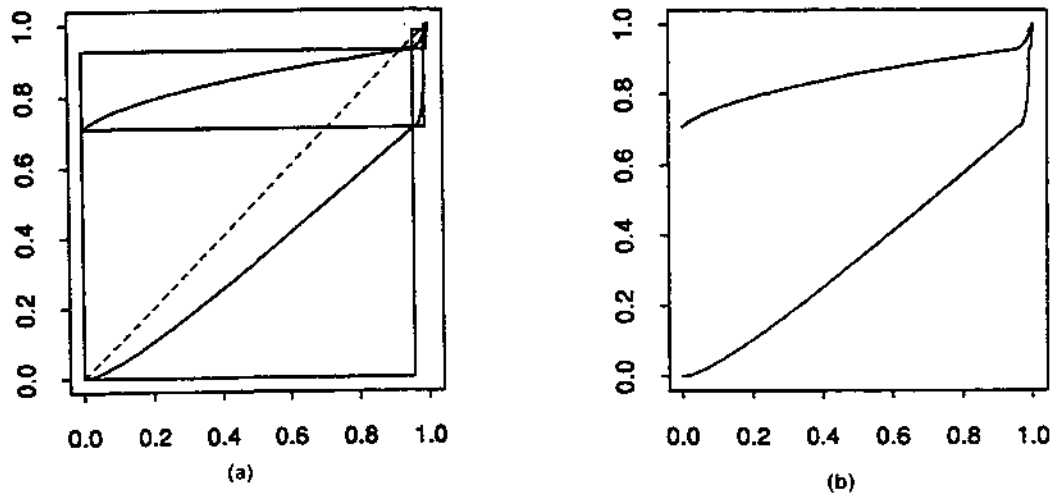
Figure 3. Example set of uniqueness for GDSM but not for DSM , as explained in the text. (a) shows the limb numbering system as well as the diagonal and boxes outlining the sets C_{2n+1} \times C_{2n} . In (b) only the limb numbering system support is shown
